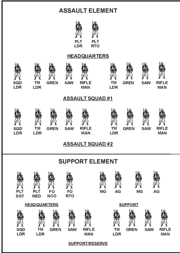
Figure 6-1. Platoon organization.
